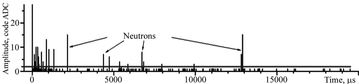
Fig. 3. Oscillogram of the detected EAS event.
