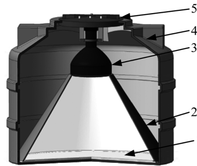
Fig. 2. Schematic diagram of the en-detector: (1) scintillator, (2) light-collecting cone, (3) FEU-200 photomultiplier, (4) light-tight box, and (5) housing cover.
