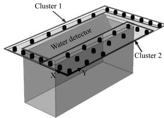
Fig. 1. Schematic diagram of the PRISMA setup.
